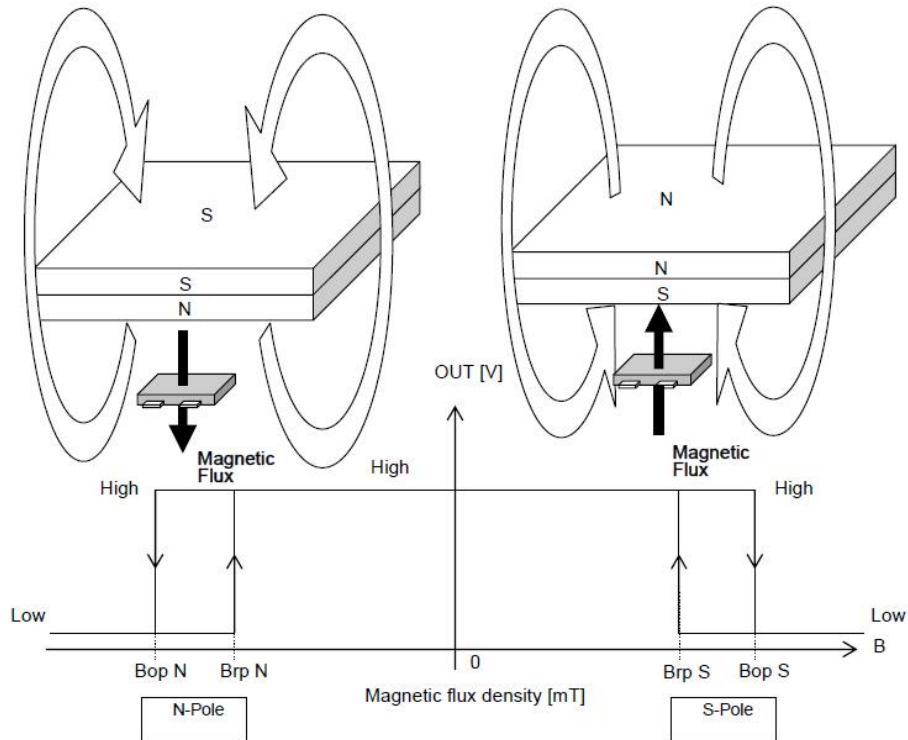
Fig 4, Magnetic Operation Characteristic of AS1801B
