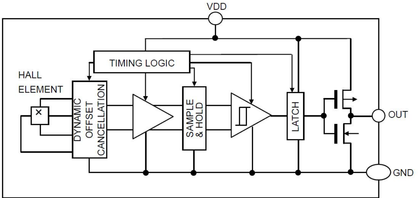
Figure 3, Block Diagram of AS1801B
